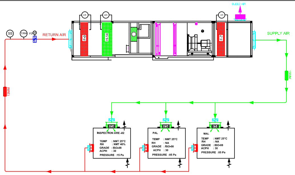
OPTION-01 : AHU WITH BREACH MODE (BIBO AT RAISER & ALSO IN AHU)
