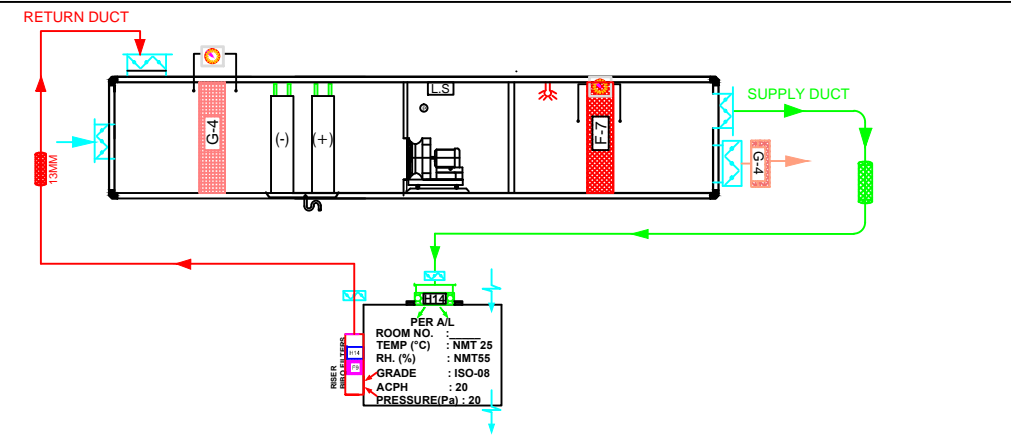
OPTION-04 : AHU WITHOUT BREACH MODE (BIBO ONLY AT RAISER)
