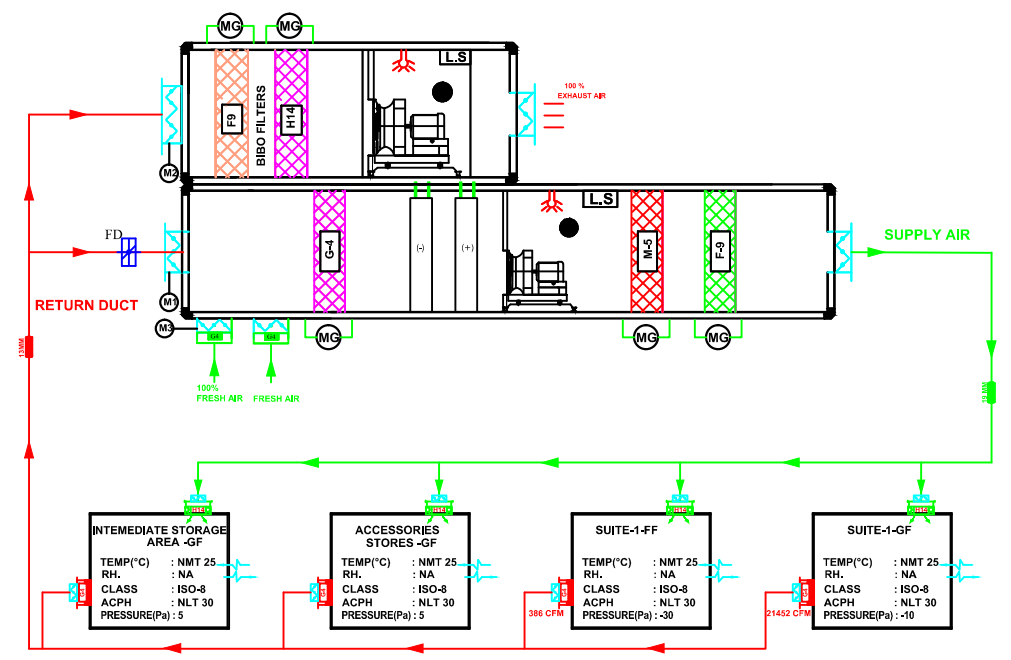
OPTION-03 : AHU WITH BREACH MODE (BIBO ONLY AT EXHAUST UNIT)
