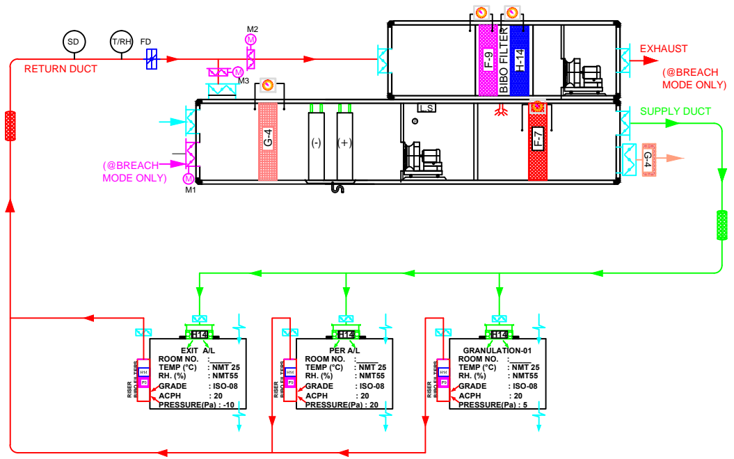
OPTION-01 : AHU WITH BREACH MODE (BIBO AT RAISER & ALSO IN AHU)
